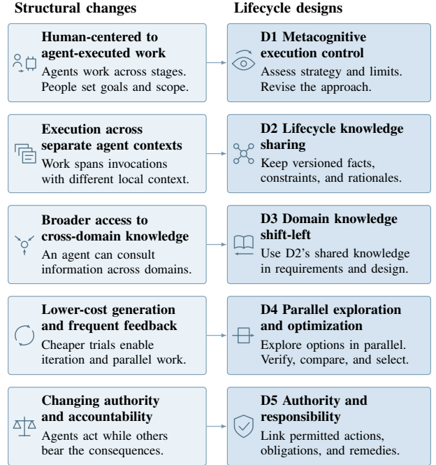
Fig. 1. Five structural changes and the five ADLC designs they motivate. Arrows show the principal correspondences.
